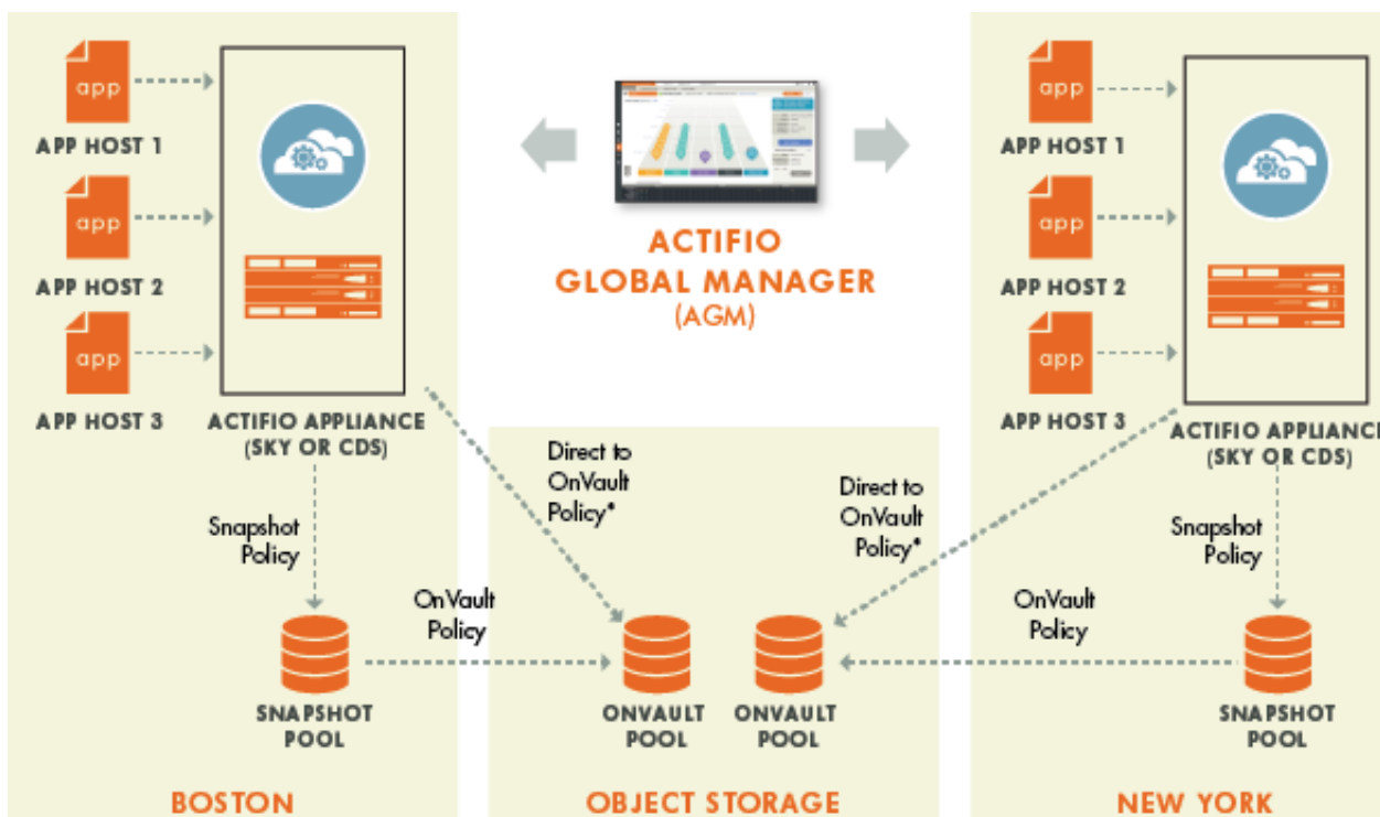
OnVault in A Multi-Actifio Appliance Environment - Managed by AGM
