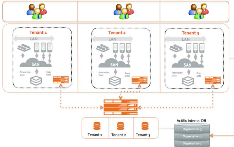
Figure 3 Role-Based Access Control per Tenant
