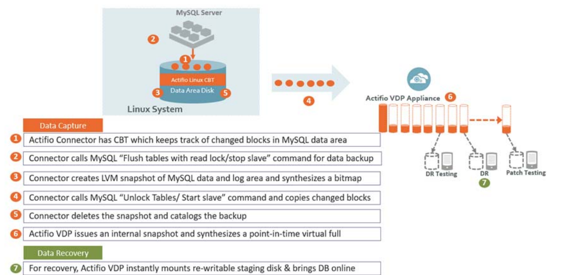
How It Works: MySQL with Linux CBT and LVM Snapshot
